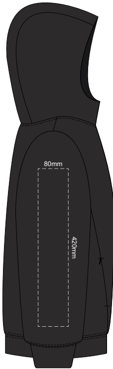
EXTRA SMALL RIGHT SLEEVE
